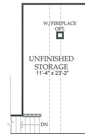
Opt. Unfinished Storage @ Attic Area
