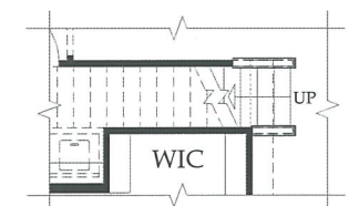
Loft Opt. @ First Floor
